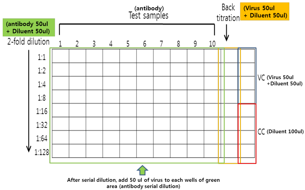
Figure 2. Serial dilution of antibody and back titration. Serial dilution of test sample (green box) and virus back titration (yellow box) is 2-fold dilution by 50 \mu l + 50 \mu l. Virus control (blue box) is also 50 \mu l + 50 \mu l, but cell control (red box) is only 100 \mu l of diluent.
