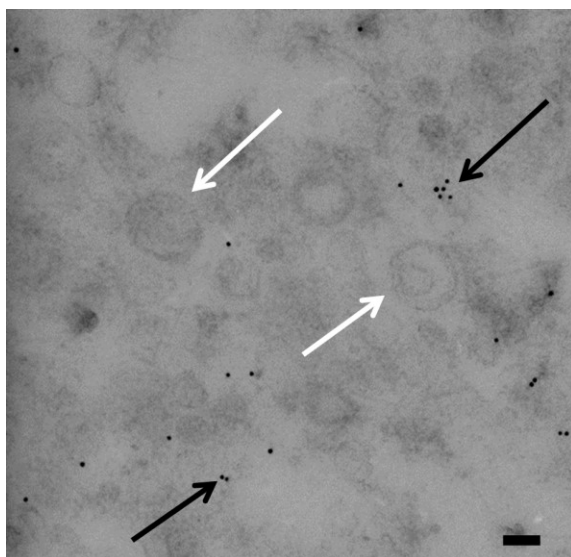
Figure 3. Transmission electron micrograph of immunogold labeling of GXM in vesicles from Bacillus subtilis . Micrograph shows vesicles and gold particles. Gold particles indicate the presence of GXM. Notice all of the gold is outside of vesicles. White arrows indicate vesicles and black arrows indicate gold particles. Scale bar = 100 nm
