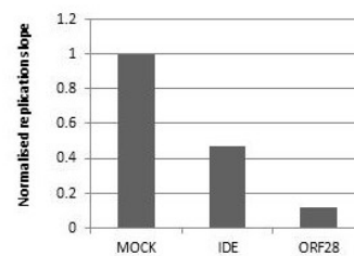
Figure 1. Calculation of replication slopes. A) Virus growth is monitored over multiple rounds of replication as a function of GFP fluorescence. B) Relative fluorescence units for mock transfected and positive controls-transfected (IDE, a cellular receptor for VZV; ORF28, the DNA polymerase for VZV) cells is plotted against hours post-infection to generate growth curve. C) The slope of replication over the linear phase of growth is calculated in Excel using the linest equation, and normalized to control (mock) transfected cells. D) Replication slopes are compared in a bar chart to see the effect of siRNA gene depletion on VZV replication.
