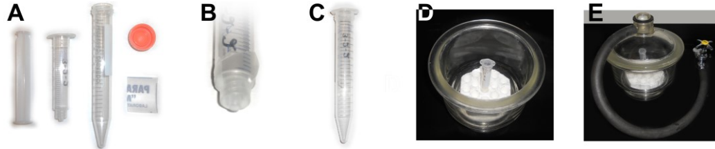
Figure 1. Apoplast extraction tools. A. Initial set: 5 ml syringe, 15 ml centrifuge tube, parafilm. B. Syringe tip sealed with parafilm. C. Syringe with sealed tip placed into centrifuge tube. D. Syringe with sealed tip in centrifuge tube placed into vacuum exicator. E. Vacuum exicator connected to the vacuum line.
